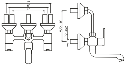
WALL MIXER 2 IN 1 MARC, DELTA WALL MIXER 3 IN 1 MARC, DELTA
