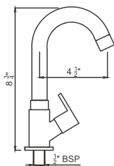
SWAN NECK REG. SPOUT MARC, DELTA, CROWN, PRIZAM
