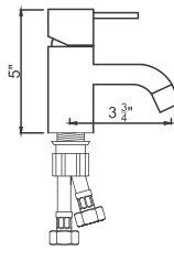
SINGLE LEVER BASIN MIXER FLORENTINE
