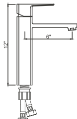
SINGLE LEVER BASIN MIXER 12" TYCOON, ROLEX
