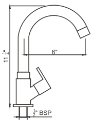
SWAN NECK PILLAR WITH EXT. SPOUT TYCOON, ROLEX
