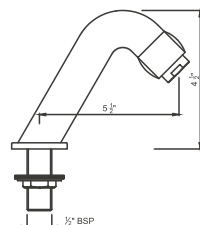
MOUTH OPERATE HIGH NECK PILLAR
