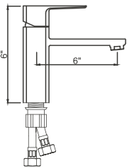
SINGLE LEVER BASIN MIXER TYCOON, ROLEX
